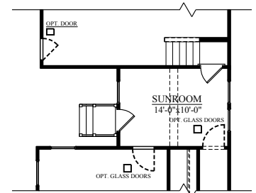
SUNROOM OPTION
