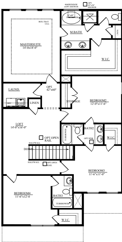
SECOND FLOOR PLANE LEVEL A
