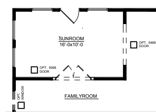
OPTIONAL SUNROOM w/ FIREPLACE 16'-0" x 10'-0"
