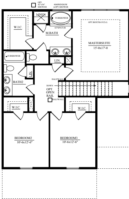
SECONDFLOORPLANELEV
