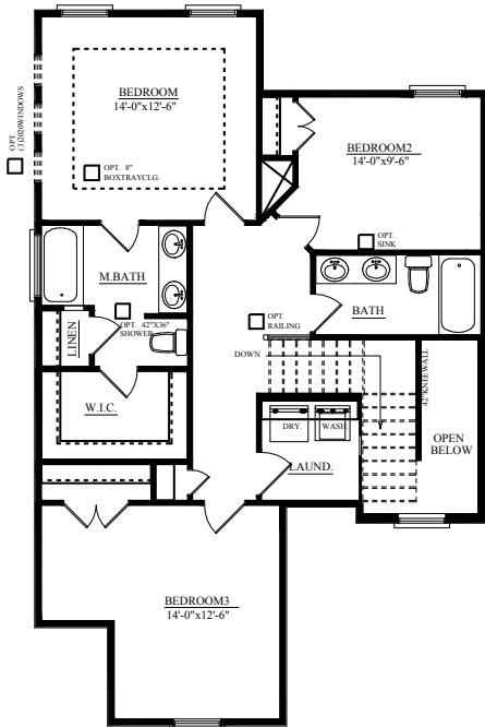
UPPER FLOOR ELEVATION A
