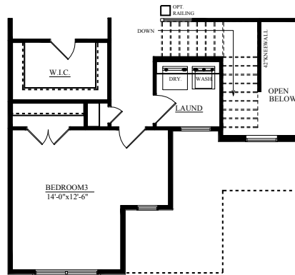
UPPER FLOOR PLAN-ELEVATION B&C
