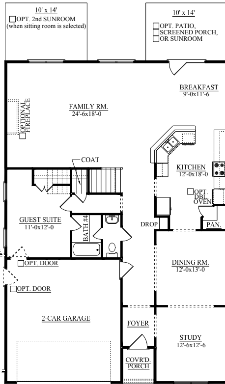
FIRST FLOOR PLAN ELEVATION "A"
