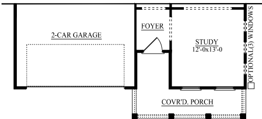
FIRST FLOOR PLAN ELEVATION "C"
