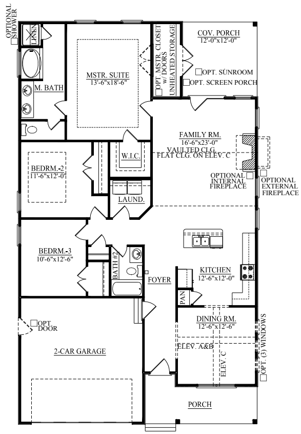
MAIN LEVEL PLAN ELEVATION A&B
