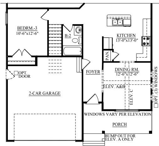
MAIN LEVEL PLAN ELEVATION (W/BONUS ROOM)
