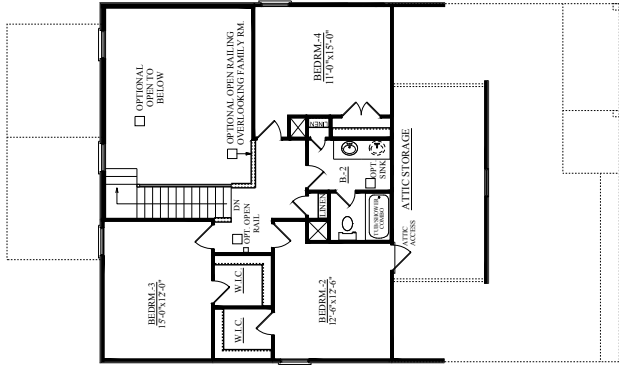
OPTIONAL SECOND FLOOR PLAN W/ BEDROOM-4
