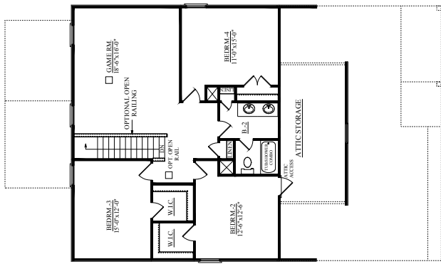
STANDARD FULL SECOND FLOOR PLAN W/ GAME RM.
