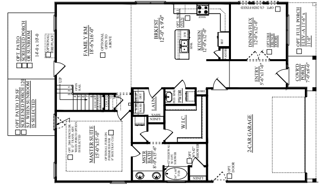
OPTIONAL SUNROOM - ADD 120 S.F. HEATED
