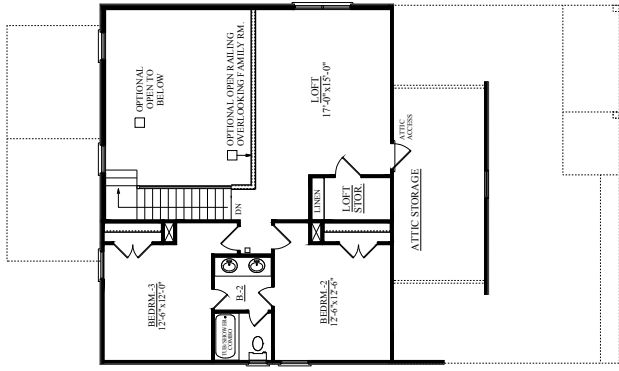
OPTIONAL OPEN SECOND FLOOR PLAN
