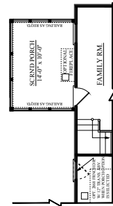
OPTIONAL SCREENED PORCH
