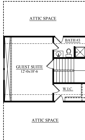
OPTIONAL 3RD FLOOR GUEST SUITE
