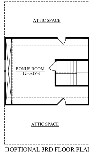
OPTIONAL 3RD FLOOR PLAN
