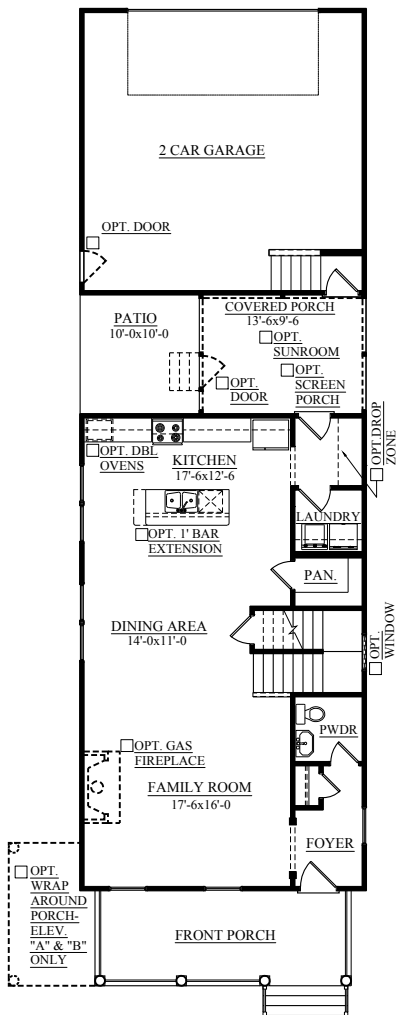
MAIN LEVEL PLAN-ELEVATION "A"
