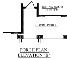
PORCH PLAN ELEVATION "B" w/ 3RD CAR
