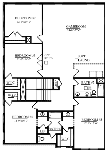
SECOND FLOOR PLAN ELEVATION A
