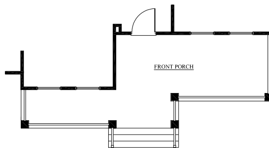
FIRST LEVEL PLAN- ELEVATION "B"
