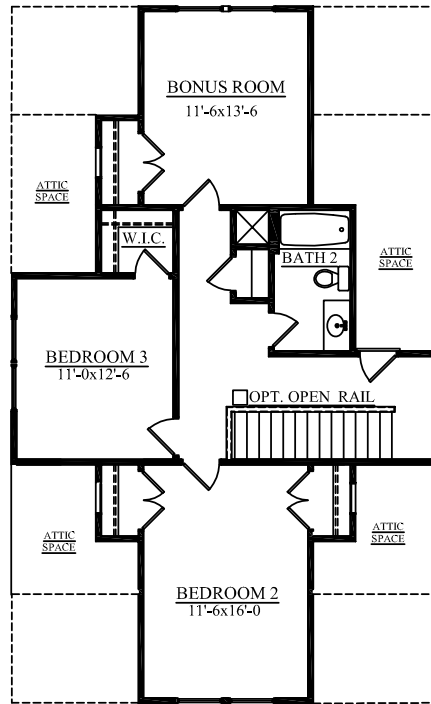
BONUS RM. UPPER LEVEL-ELEV. A
