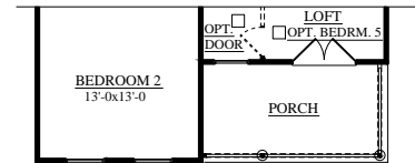
PARTIAL SECOND FLOOR PLAN ELEV. B
