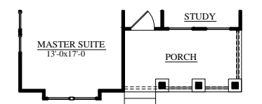
PARTIAL FIRST FLOOR PLAN ELEV. F
