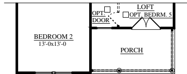
PARTIAL SECOND FLOOR PLAN ELEV. D
