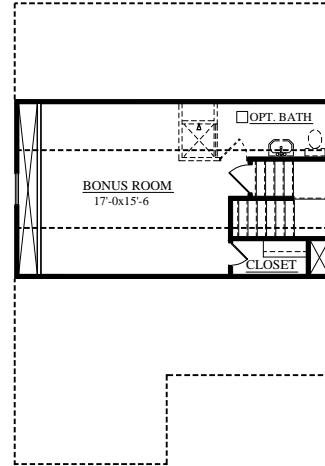
THIRD FLOOR PLAN ELEV. B,D & G
