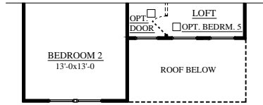
PARTIAL SECOND FLOOR PLAN ELEV. F&G
