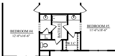
□ SECOND FLOOR PLAN ELEVATION C
