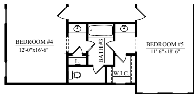
□ SECOND FLOOR PLAN ELEVATION B
