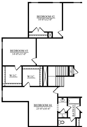
□ SECOND FLOOR PLAN W/ 3 CAR DELUXE
