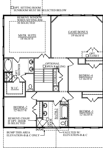
STANDARD SECOND FLOOR PLAN
