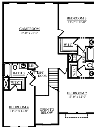
ELEVATION A-SECOND FLOOR PLAN
