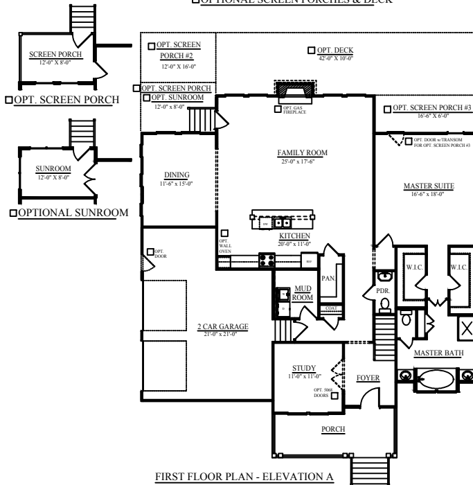
FIRST FLOOR PLAN - ELEVATION A
