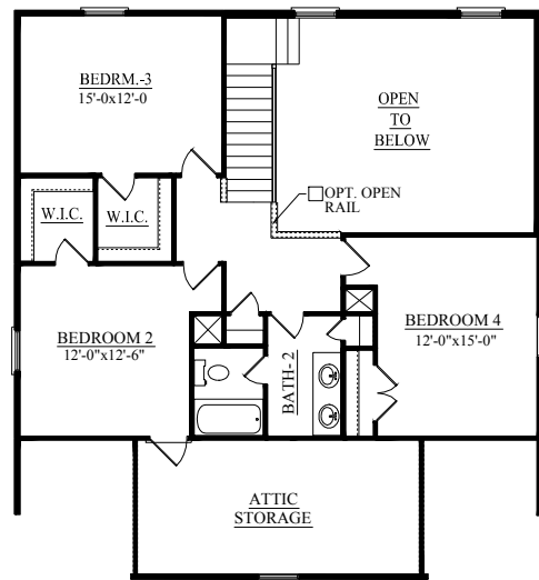
OPTIONAL SECOND FLOOR PLAN w/ 2-STORY FAMILY ROOM
