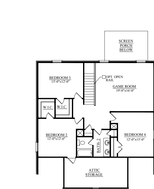
STANDARD FULL SECOND FLOOR PLAN W/ GAME RM.
