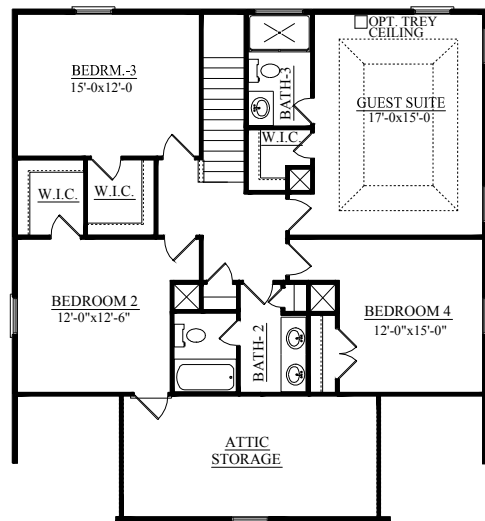
OPTIONAL FULL SECOND FLOOR PLAN W/ GUEST SUITE
