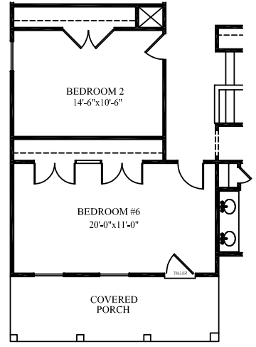
BEDROOM #6 OPTION SECOND FLOOR PLAN - B
