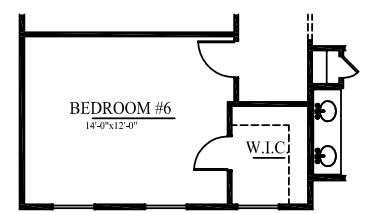
BEDROOM #6 OPTION SECOND FLOOR PLAN - C
