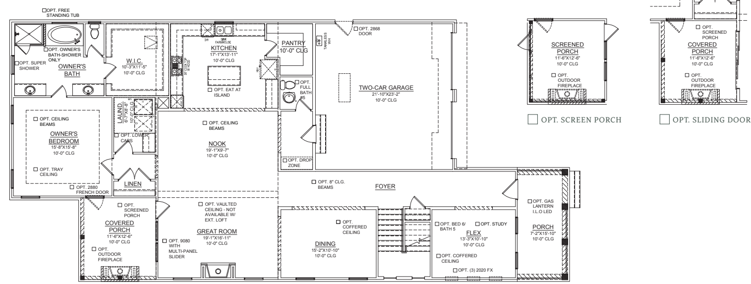
FIRST FLOOR PLAN ELEVATION C
