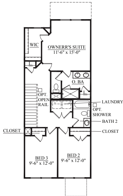
SECOND FLOOR PLAN ELEVATION C
