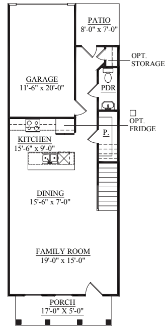
FIRST FLOOR PLAN ELEVATION D
