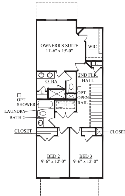
SECOND FLOOR PLAN ELEVATION D
