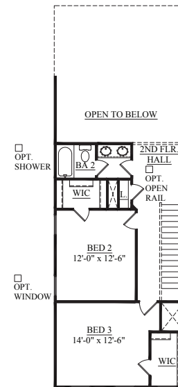
SECOND FLOOR PLAN ELEVATION C
