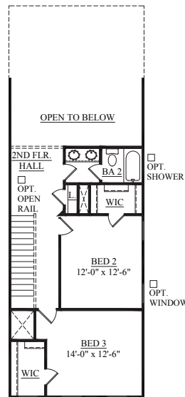
SECOND FLOOR PLAN ELEVATION B
