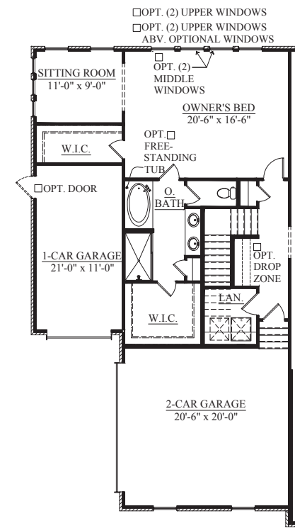
OPT. 3RD CAR GARAGE W/ SITTING ROOM ELEVATION A
