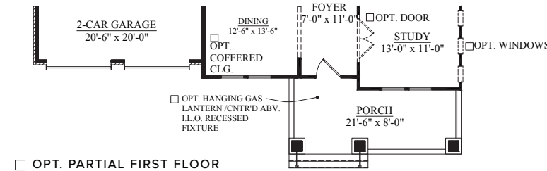
OPT. PARTIAL FIRST FLOOR ELEVATION B
