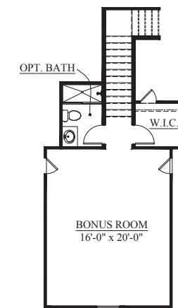
OPT. BONUS LEVEL PLAN
