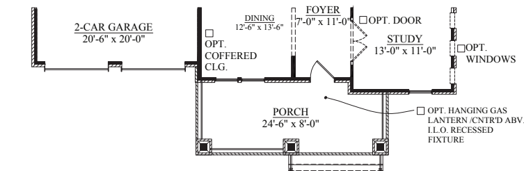
OPT. PARTIAL FIRST FLOOR ELEVATION C
