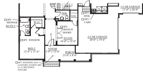
FIRST FLOOR PLAN ELEVATION C
