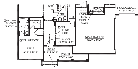
FIRST FLOOR PLAN ELEVATION D
