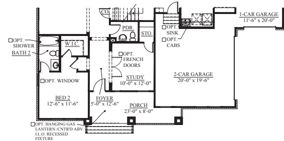
FIRST FLOOR PLAN ELEVATION B
