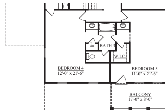
SECOND FLOOR PLAN ELEVATION C
