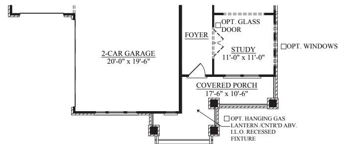
FIRST FLOOR PLAN ELEVATION B
