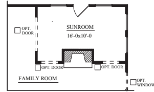
OPT. SUNROOM WITH FIREPLACE
