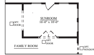
OPT. SUNROOM WITHOUT FIREPLACE
