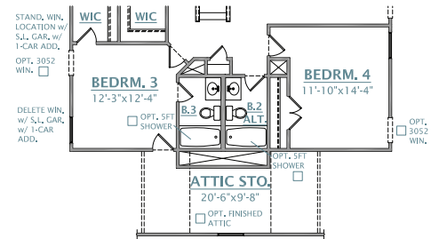
OPT. SECOND FLOOR PLAN WITH BATH #3 OPT. ELEVATION A, B, C
