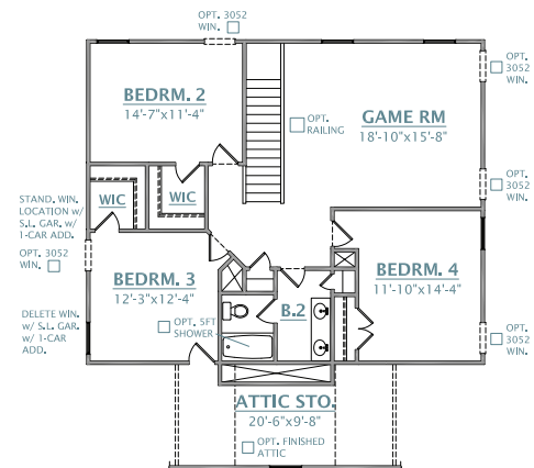
SECOND FLOOR PLAN ELEVATION A, B, C
