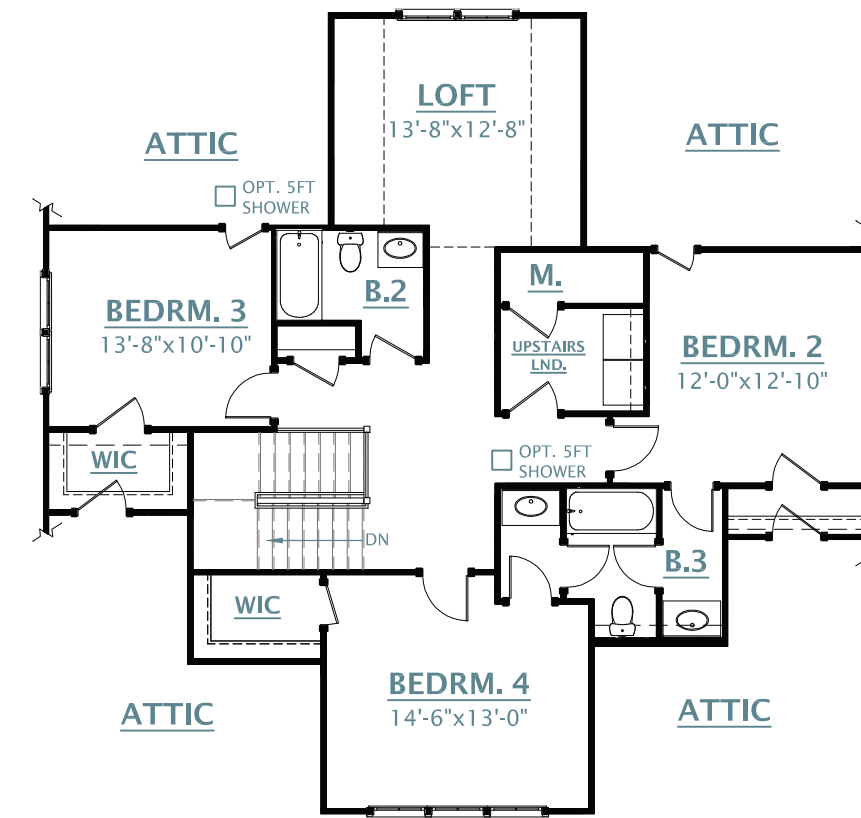
STANDARD SECOND FLOOR PLAN
