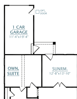
OPT. 1 CAR REARLOAD GARAGE WITH SUNROOM
