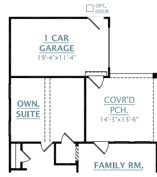
OPT. 1 CAR SIDELOAD GARAGE WITH COVERED PORCH
