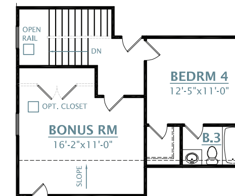
OPT. BONUS ROOM WITH BEDROOM 4 SUITE
