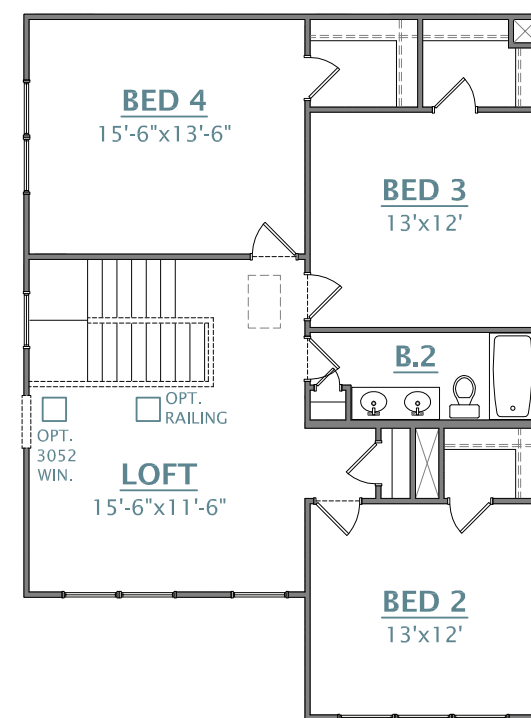
SECOND FLOOR PLAN ELEVATION A
