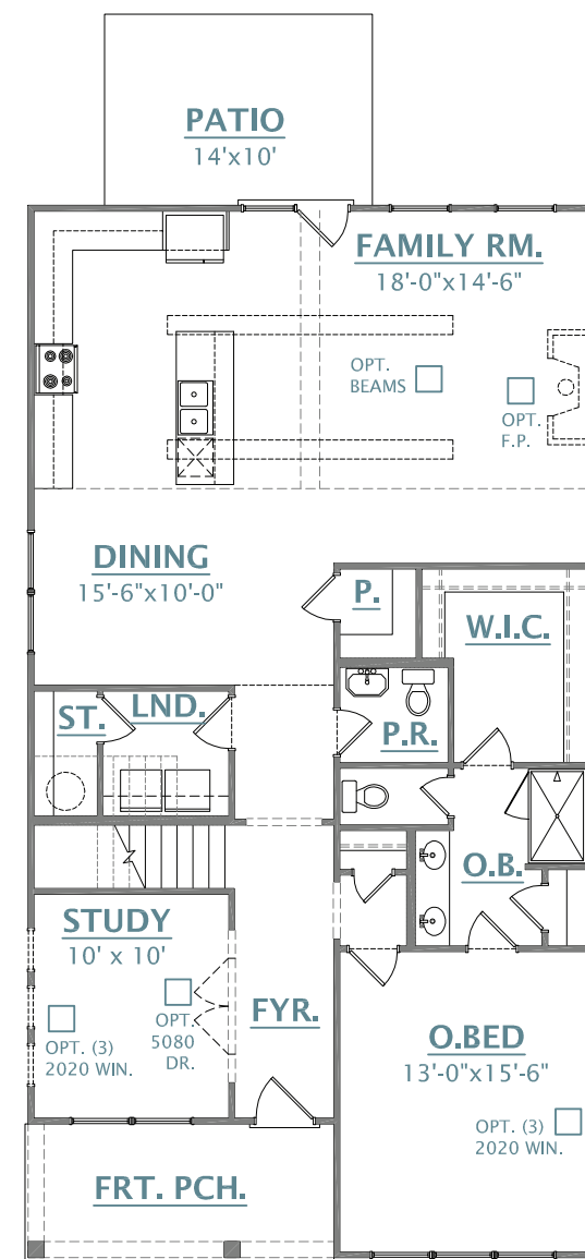
FIRST FLOOR PLAN ELEVATION A
