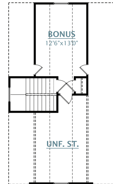
OPT THIRD LEVEL PLAN ELEVATIONS A & B ONLY
