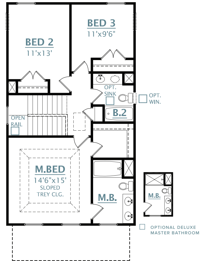
OPT THIRD LEVEL PLAN ELEVATIONS A & B ONLY
