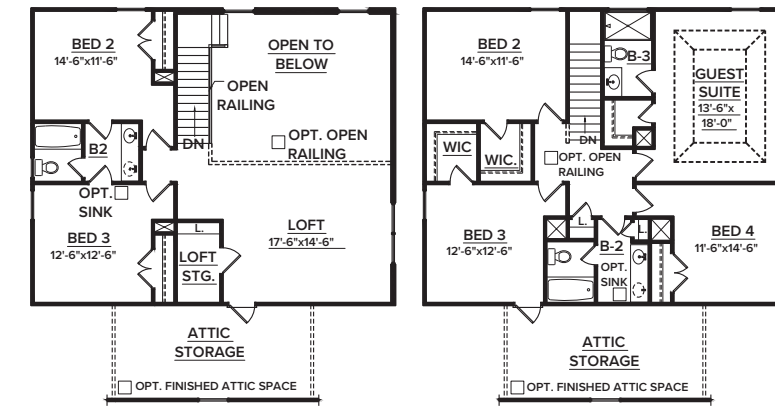
OPT. SECOND FLOOR WITH LOFT
