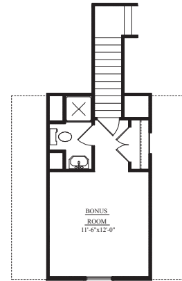
OPTIONAL BONUS ROOM WITH BATH
