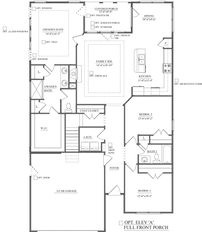
MAIN LEVEL PLAN
