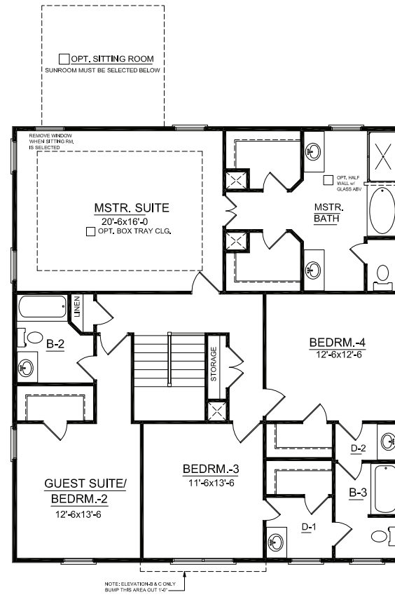
OPT. FULL SECOND FLOOR PLAN WITH ENLARGED MASTER AREA, GUEST SUITE & BATH
