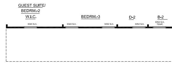
SECOND FLOOR PLAN ELEVATION D
