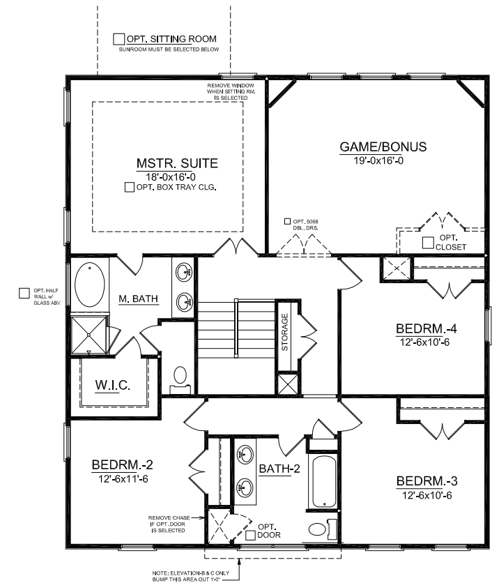
STANDARD SECOND FLOOR PLAN
