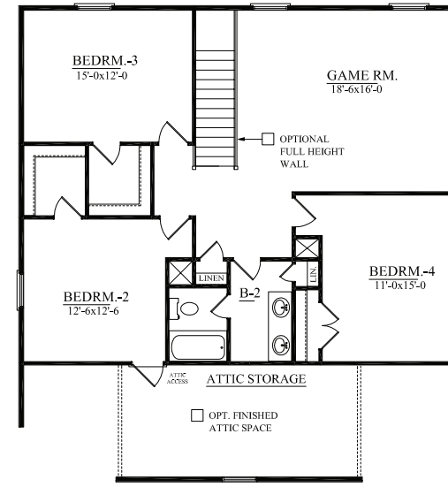
STANDARD FULL SECOND FLOOR PLAN WITH GAMEROOM
