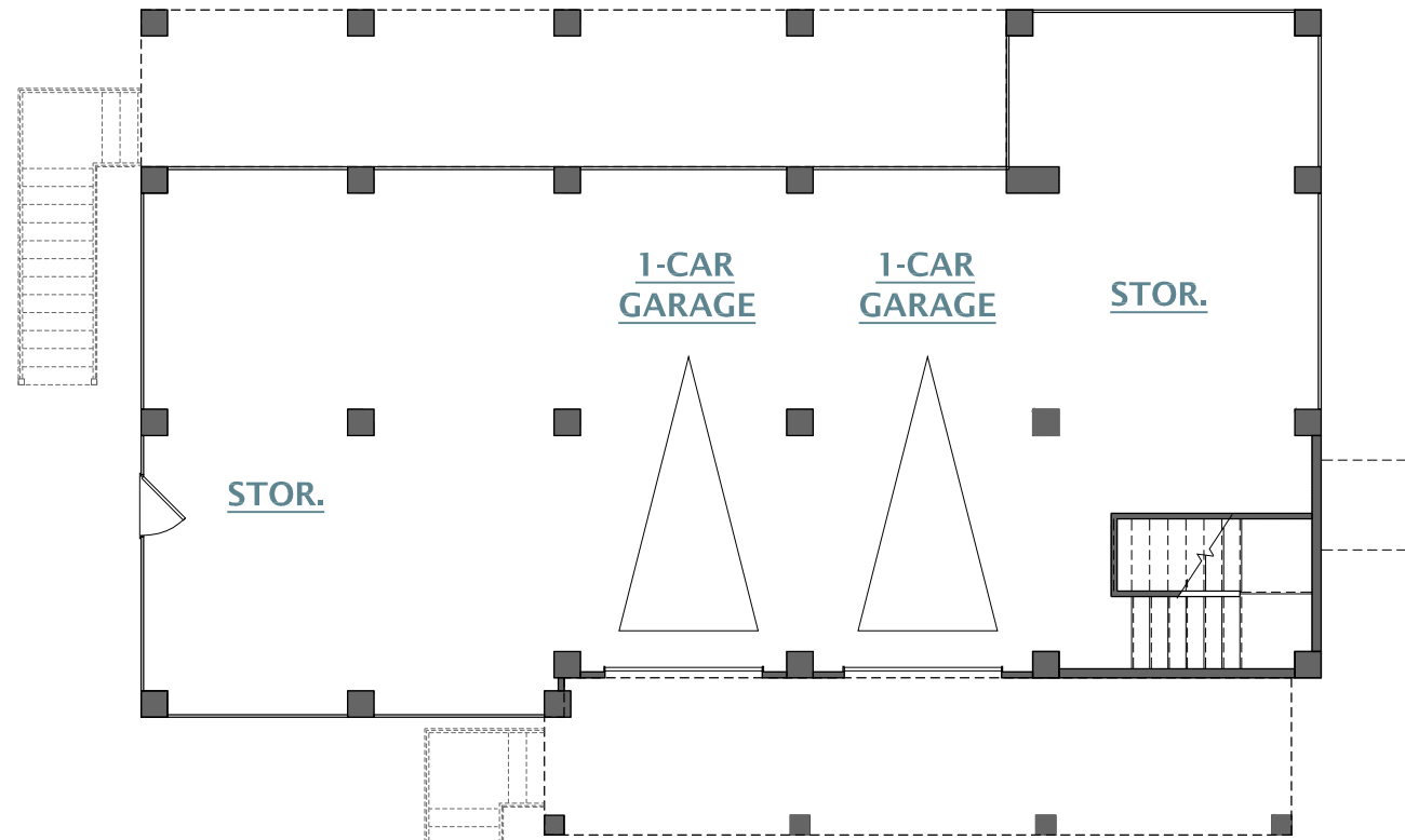
GARAGE LEVEL PLAN ELEVATION "A & B"
