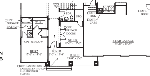
FIRST FLOOR PLAN ELEVATION B
