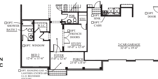
FIRST FLOOR PLAN ELEVATION C
