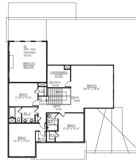
SECOND FLOOR PLAN ELEVATION D
