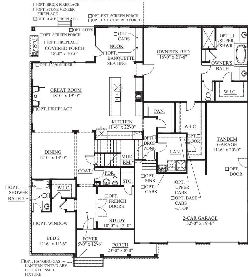
FIRST FLOOR PLAN ELEVATION A
