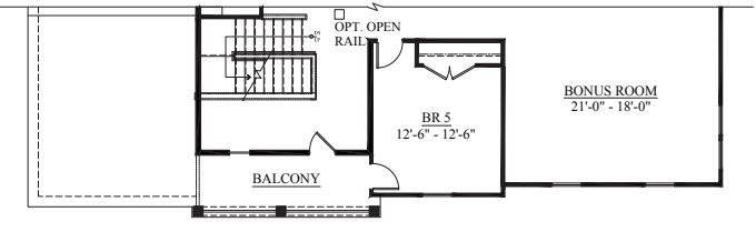
OPT. SECOND FLOOR PLAN ELEVATION C
