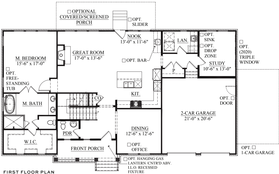
FIRST FLOOR PLAN ELEVATION A
