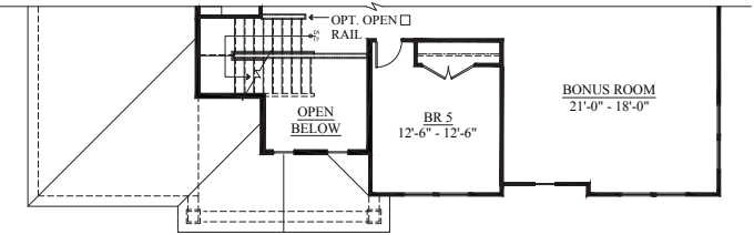
OPT. SECOND FLOOR PLAN ELEVATION B
