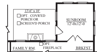
OPTIONAL SUNROOM ADDS +120 HEATED SQ FT
