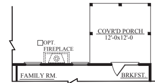
OPT. COVERED PORCH
