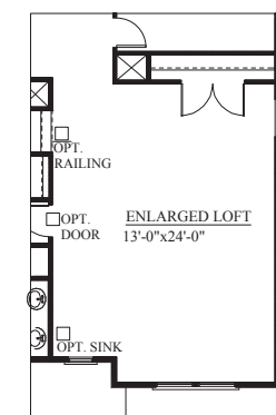
OPT. ENLARGED LOFT
