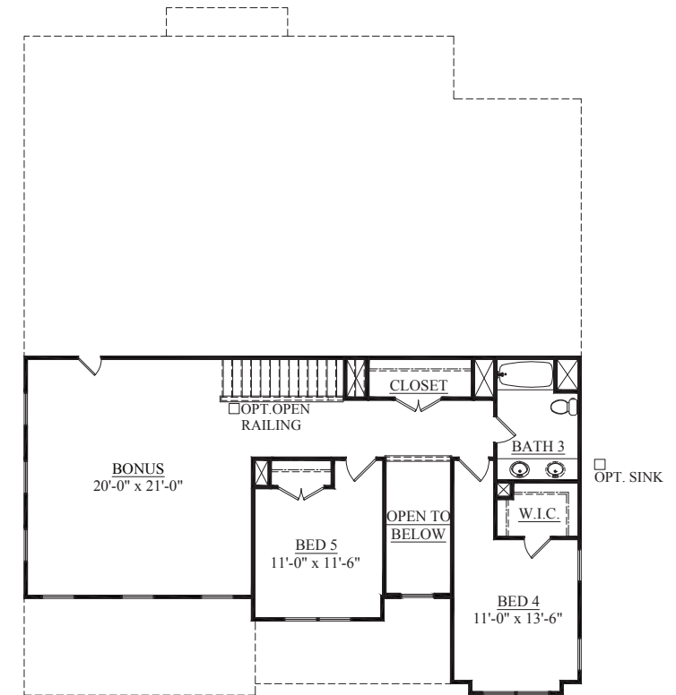
SECOND FLOOR PLAN ELEVATION A
