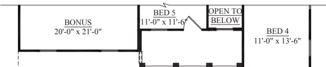
□ SECOND FLOOR PLAN ELEVATION D
