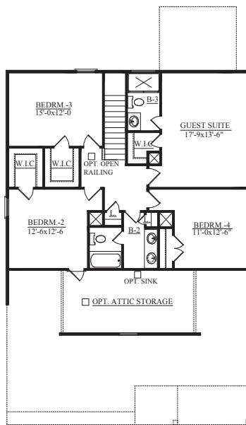
OPTIONAL FULL SECOND FLOOR PLAN WITH GUEST SUITE
