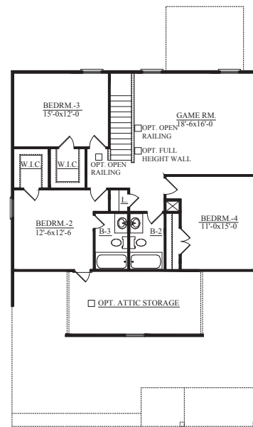
STANDARD FULL SECOND FLOOR PLAN WITH GAME ROOM / 2 BATHS
