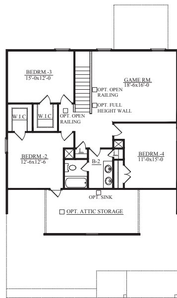
STANDARD FULL SECOND FLOOR PLAN WITH GAME ROOM
