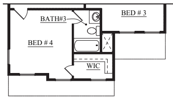
SECOND FLR. PLAN ELEVATION B
