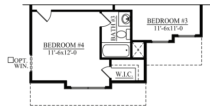
SECOND FLOOR PLAN ELEVATION C
