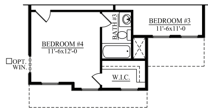
SECOND FLOOR PLAN ELEVATION B
