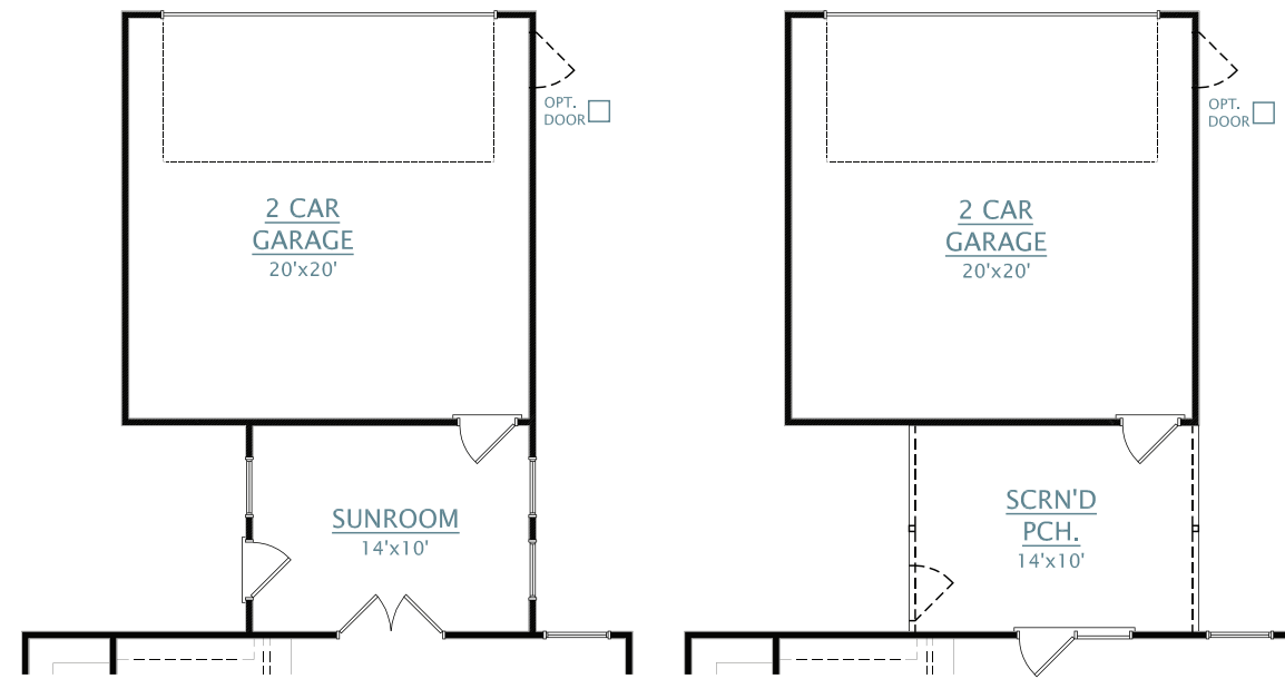
OPT. 2 CAR GARAGE ATTACHED BY SUNROOM
