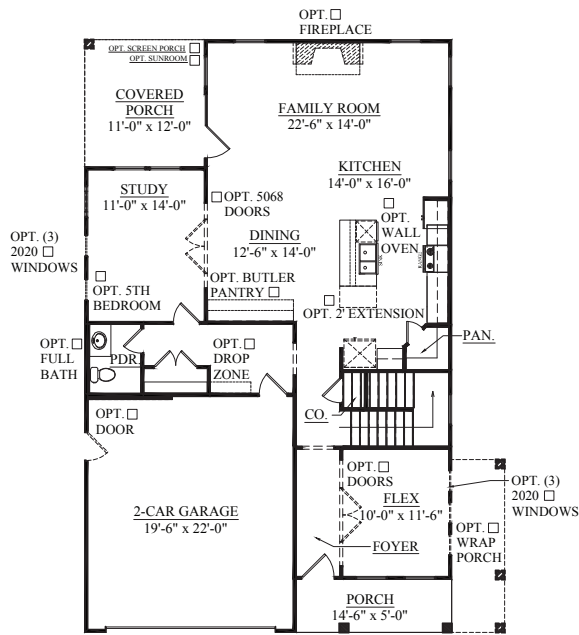
FIRST FLOOR PLAN ELEVATION A.C
