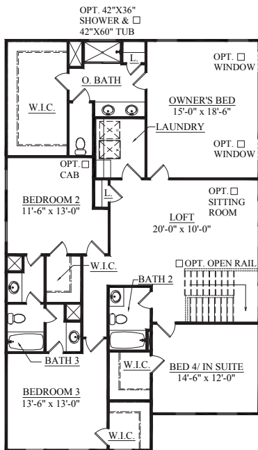
SECOND FLOOR PLAN ELEVATION A
