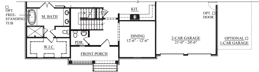
OPT. FIRST FLOOR PLAN ELEVATION C
