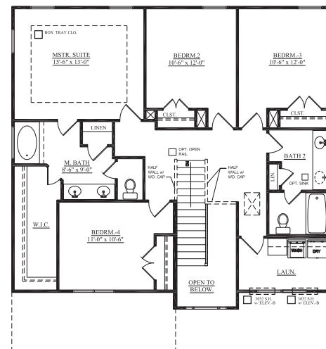
SECOND FLOOR PLAN ELEVATION A
