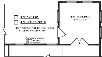
OPT. SUNROOM ADD 120 SF HEATED
