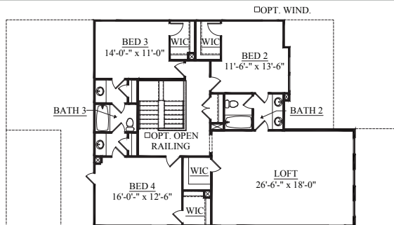
SECOND FLOOR PLAN ELEVATION A, C
