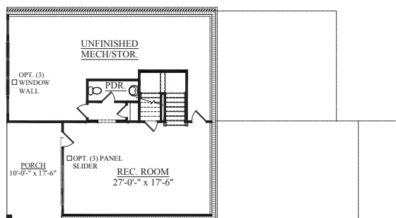
OPT. BASEMENT PLAN W/ REC ROOM AND STORAGE
