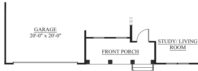
FIRST FLOOR PLAN ELEVATION C
