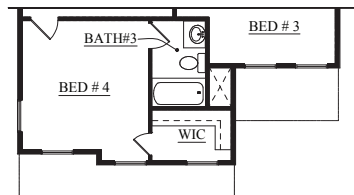
SECOND FLR. PLAN ELEVATION B
